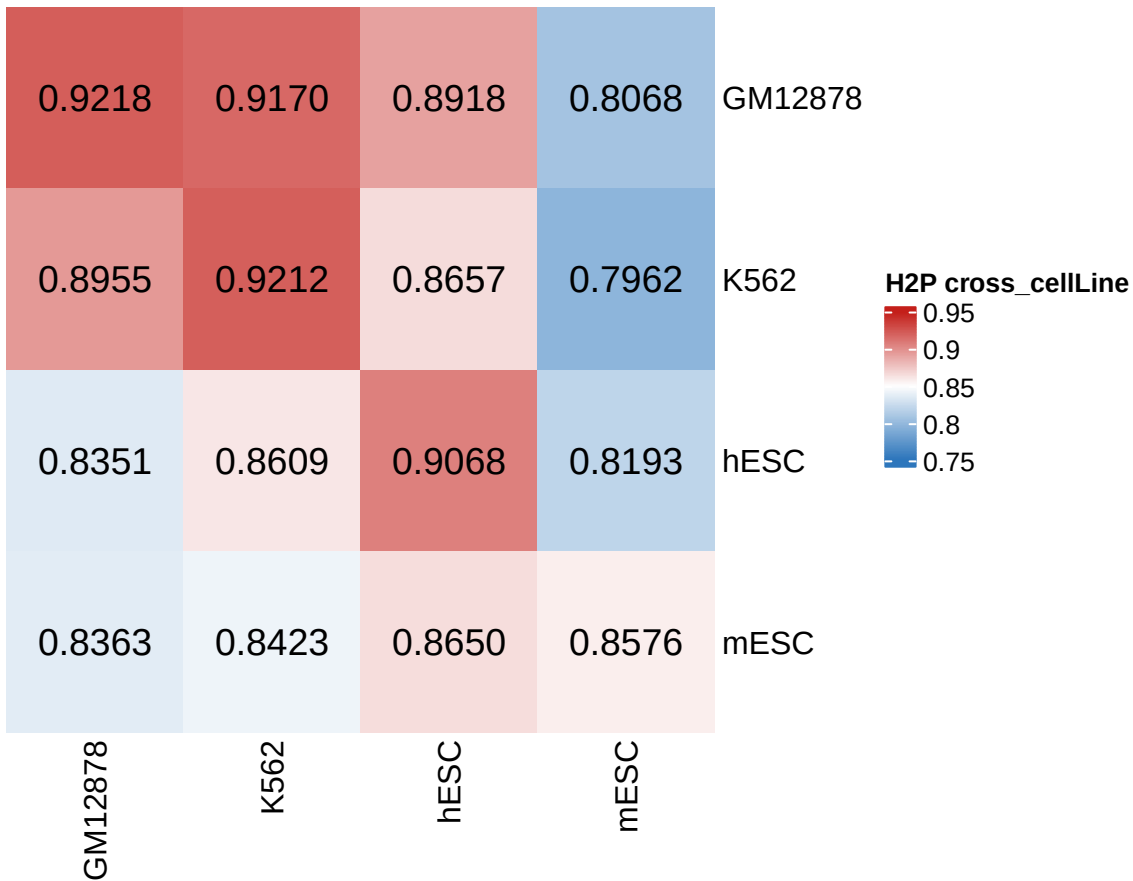
H2P Cross cellLine prediction (100kb)
